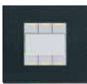
dark rock
