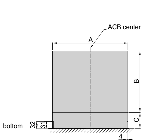
Rear panel cutting size (mm)
