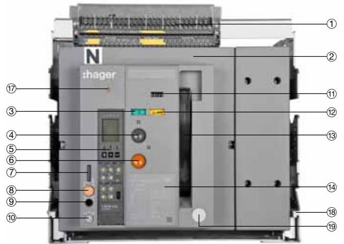
Draw-out type
