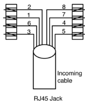
RJ45 Jack pin. EIA/TIA 568B EIA/TIA 568A
